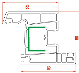
Super Sash Profile
