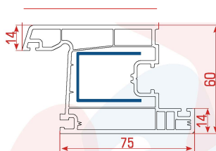
Narrow Inside Opening Door Sash Profile
