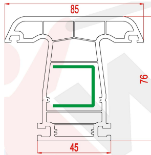
Mullion Profile
