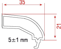
Single Glazing Bead Profile
