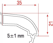
Single Glazing Bead Profile Tek Cam Çita Profili
