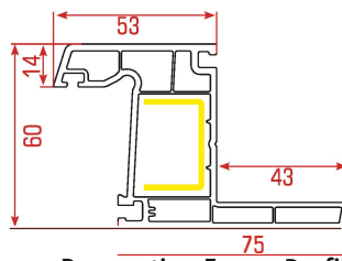
Renovation Frame Profile
