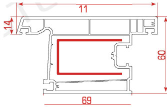
Outside Opening Door Sash Profile
