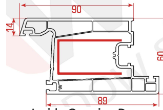
Inside Opening Door Sash Profile
