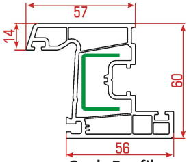
Sash Profile
