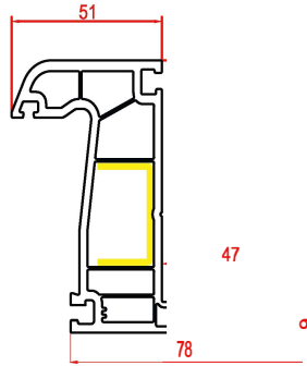
Renovation Frame Profile
