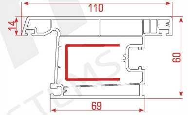
Outside Opening Door Sash Profile
