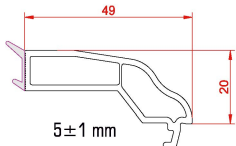
Single Glazing Bead Profile
