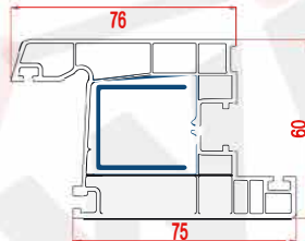
Narrow Inside Opening Door Sash Profile
