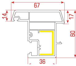
Moving Mullion Profile
