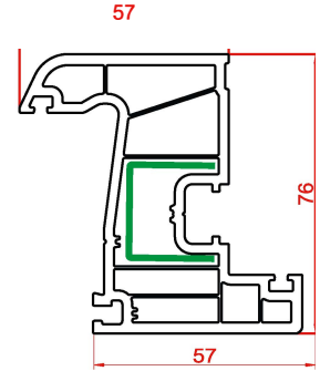
Sash Profile
