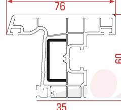
Outside Opening Window Sash Profile
