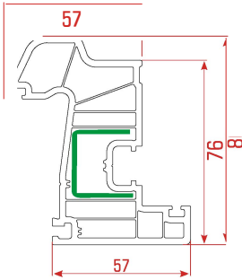
Drainaged Sash Profile
