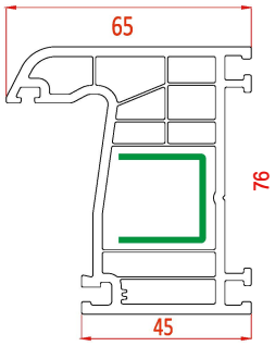
Frame Profile
