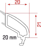
Double Glazing Bead Profile
