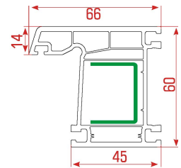
Super Frame Profile
