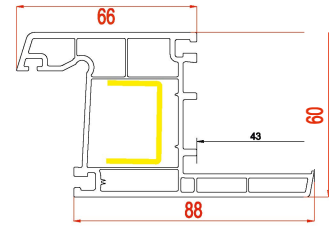
Renovation Super Frame Profile
