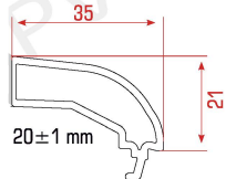
Single Glazing Bead Profile
